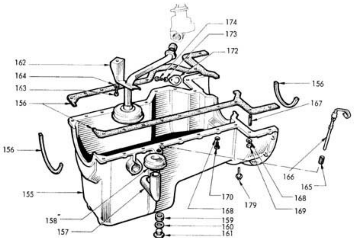
4 CYLINDER FRONT WELL SUMP
