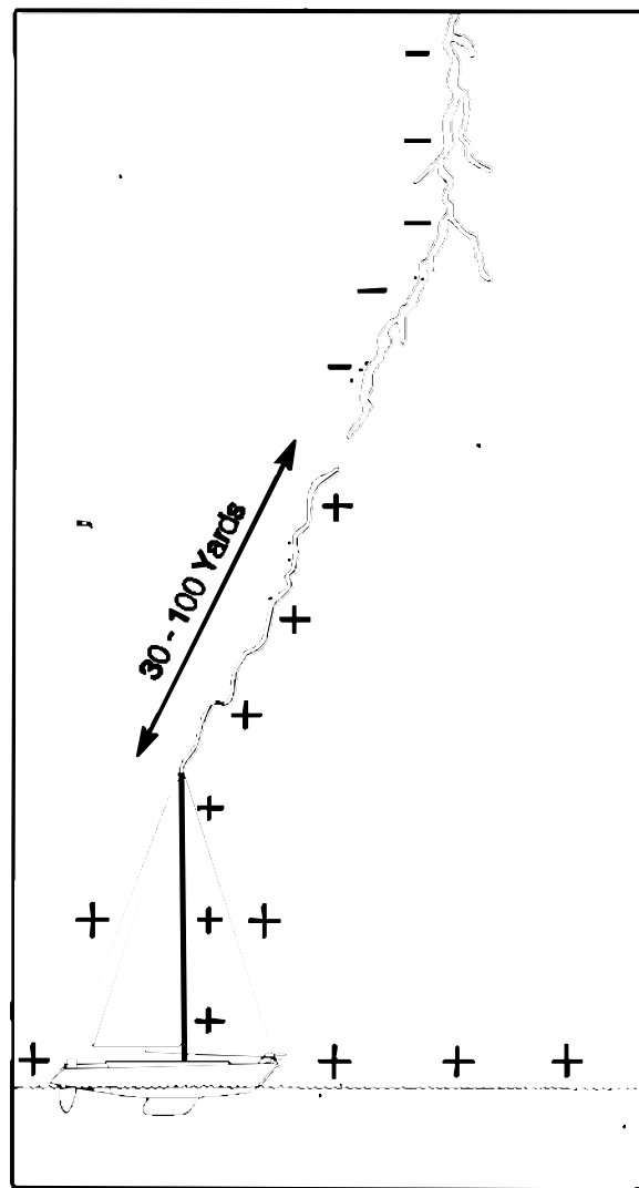
Figure 2. Lightning attachment to a sailboat.
